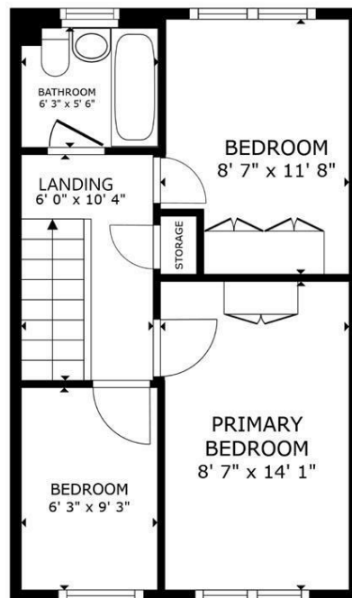
FLOOR 2
